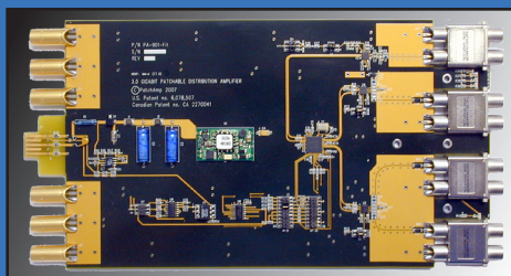
PA901 DA with patches
